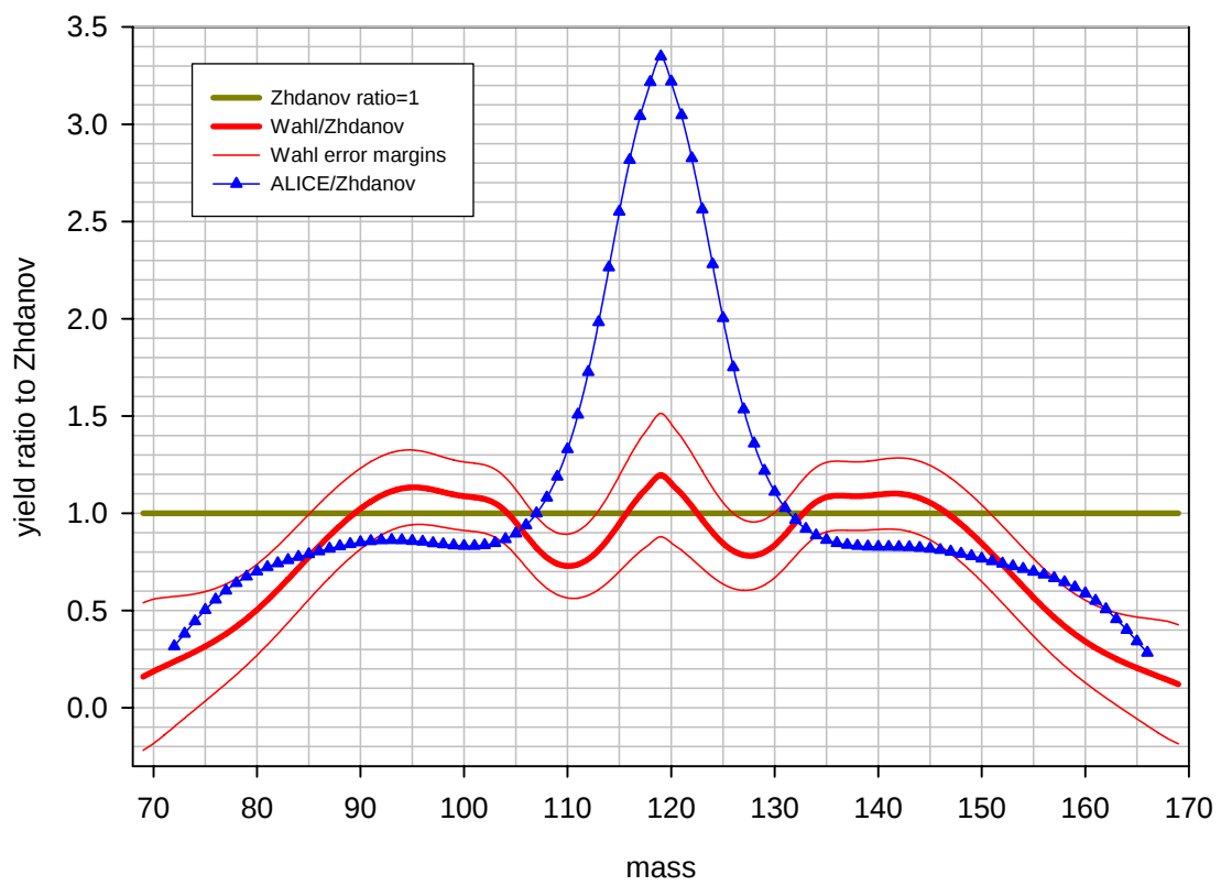
Benchmark B: ^{237}\text{Np} at 13 MeV, pre-neutron emission yield ratio to Zhdanov's data
